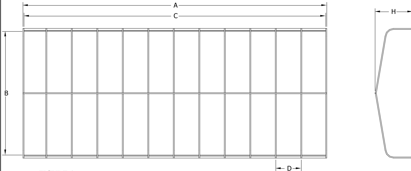
FIGURE 1 *ALL MEASUREMENTS (±1")
