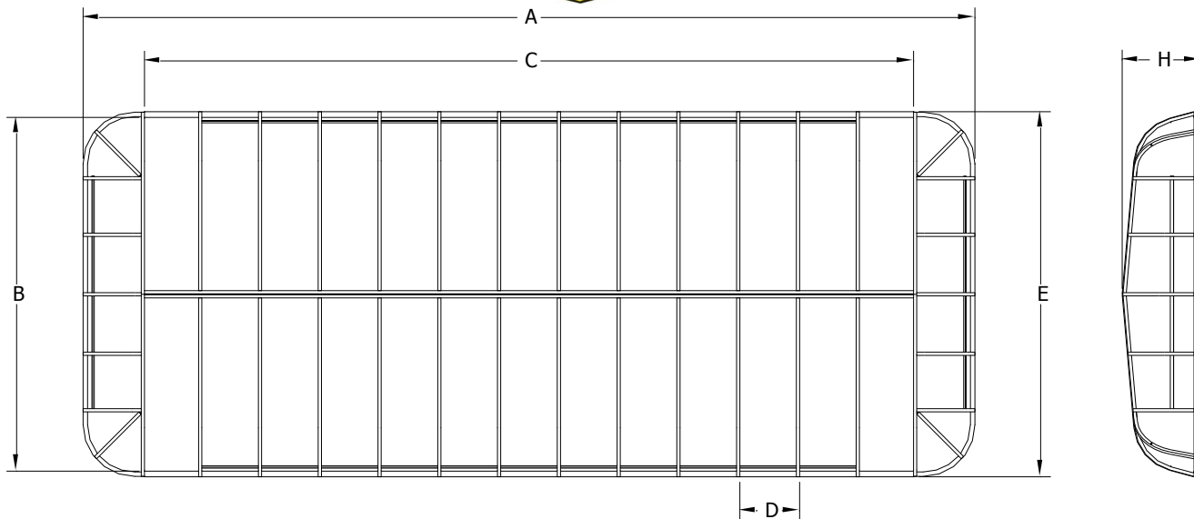
FIGURE 1 *ALL MEASUREMENTS (±1")
