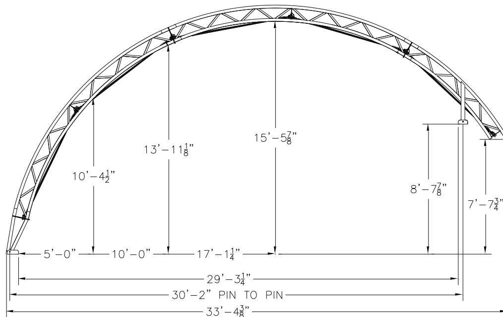
INTERIOR CLEARANCE
